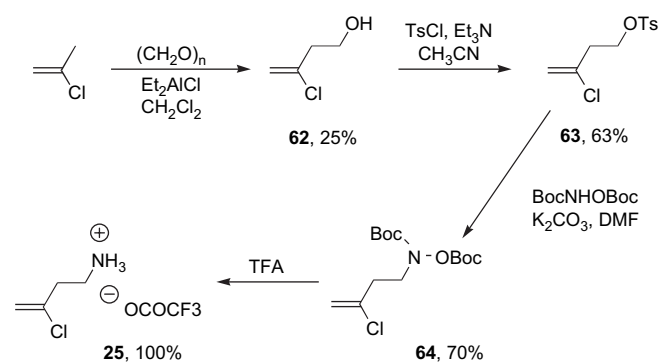
Scheme 15.
