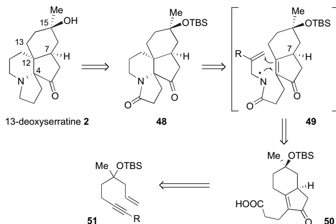
Scheme 12.
