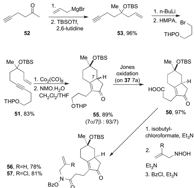
Scheme 13.
