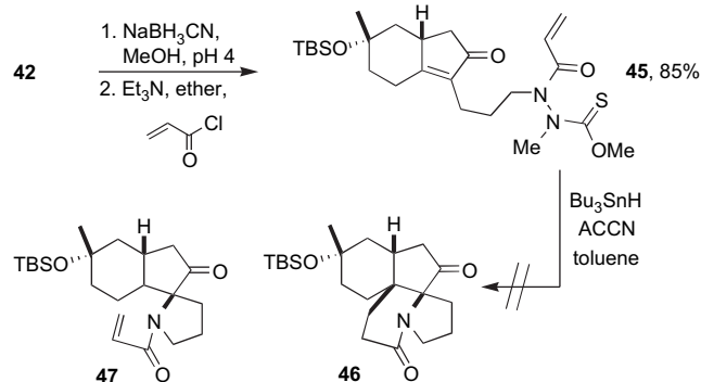
Scheme 11.
