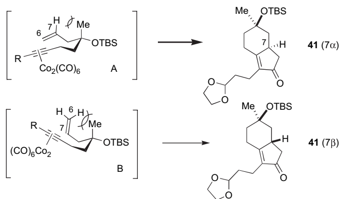
Scheme 10.
